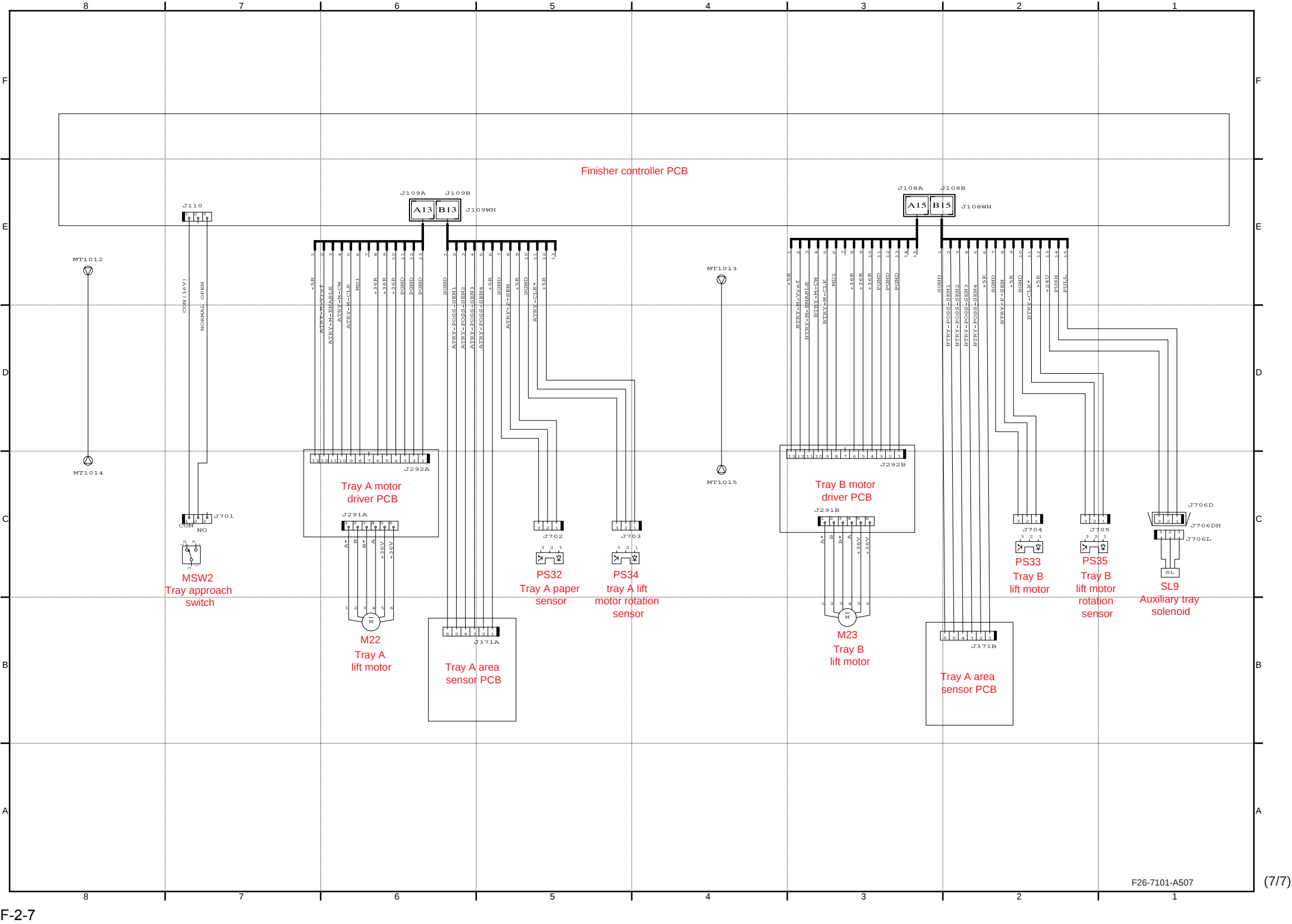
General Circuit Diagram(Finisher7)
