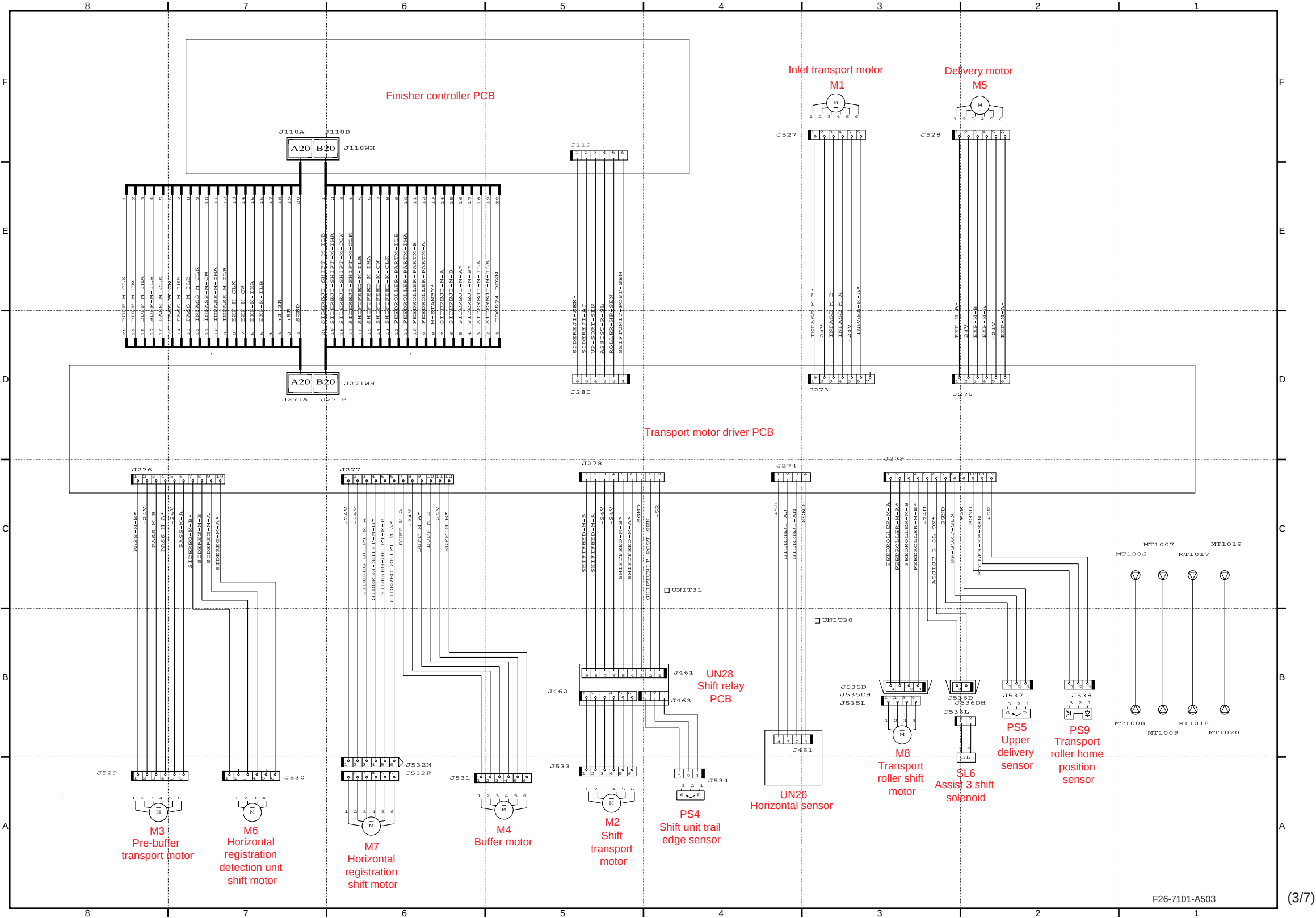
General Circuit Diagram(Finisher3)
